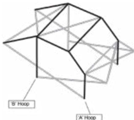
Drawing.8.1 ROPS
