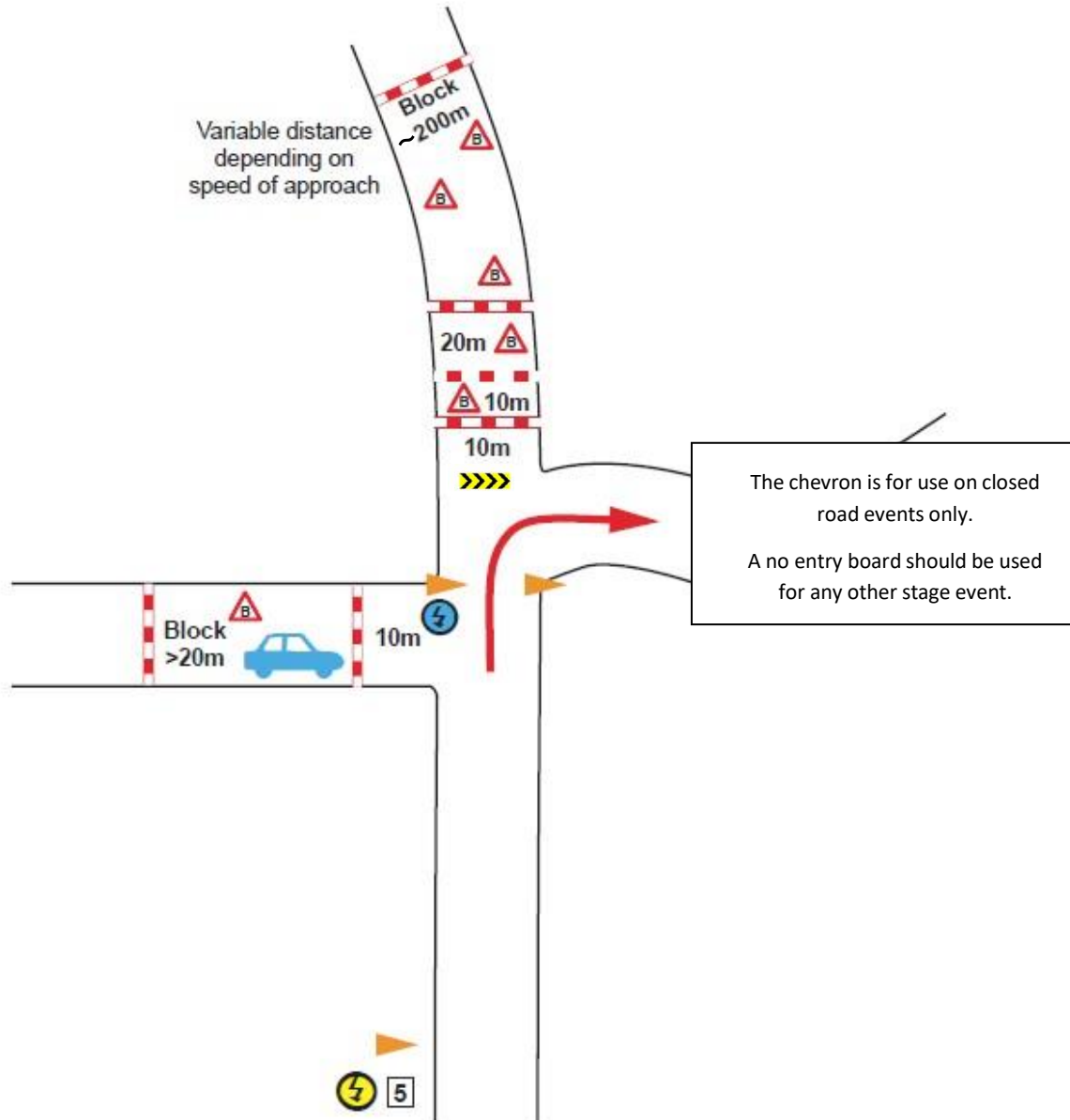
Alternative to Drawing No. 29 without the use of box junctions
